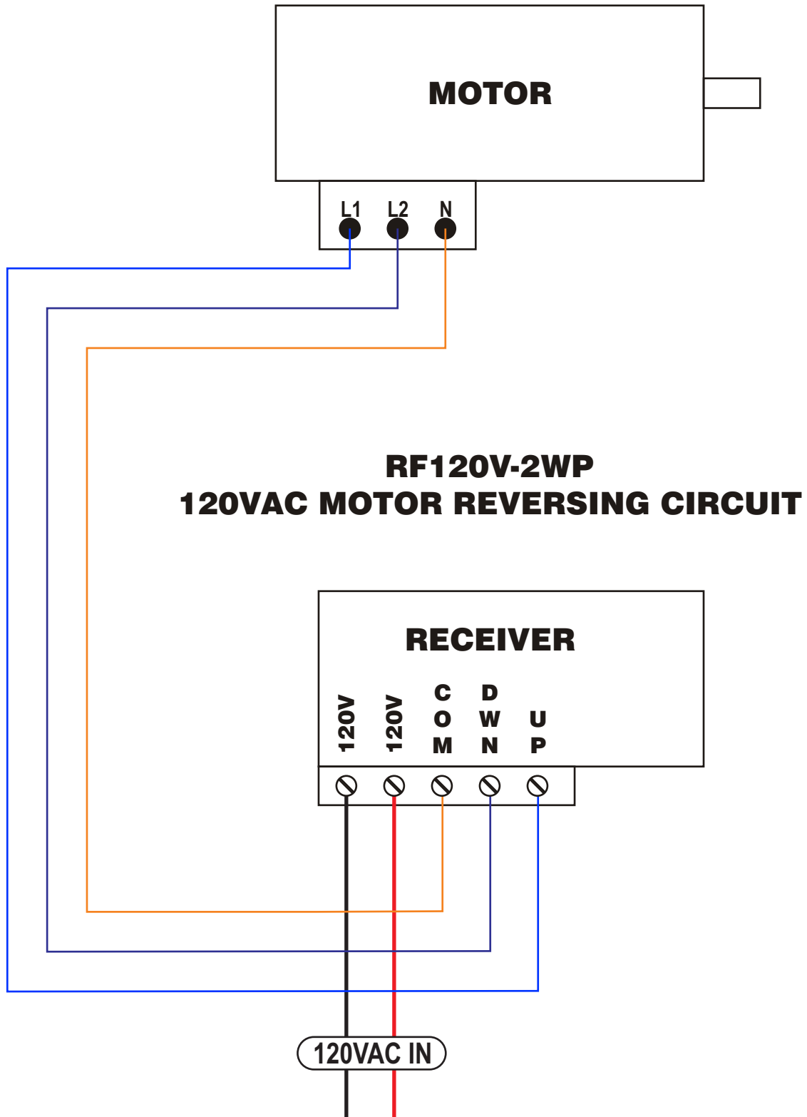
RF120V-2WP WIRING DIAGRAM
